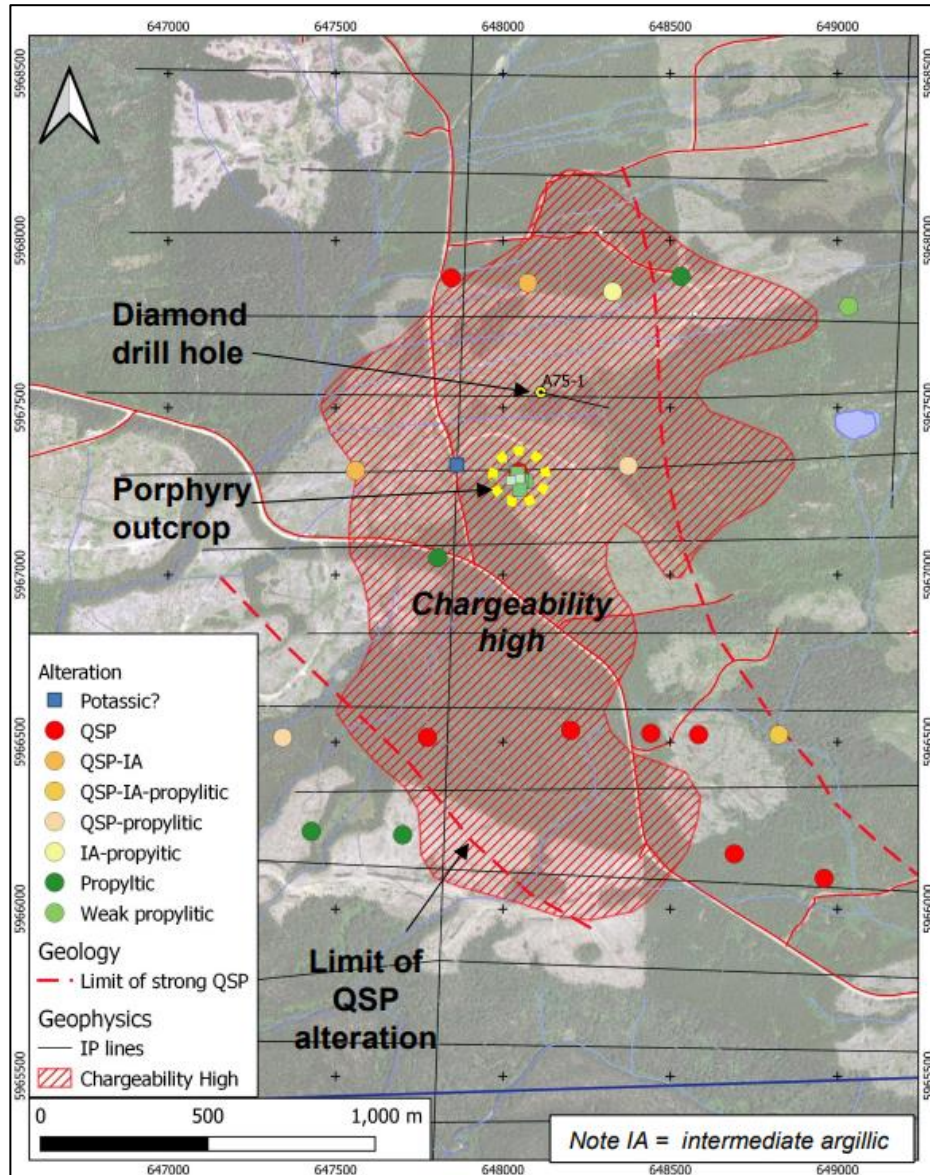
Figure 1. A large historically delineated IP chargeability high with areas of alteration, as defined from percussion drilling logs, a diamond drill hole, and outcrop, and the extent of strong quartz-sericite-pyrite (QSP) alteration, provide for an immediate target area for exploration and future drilling.
